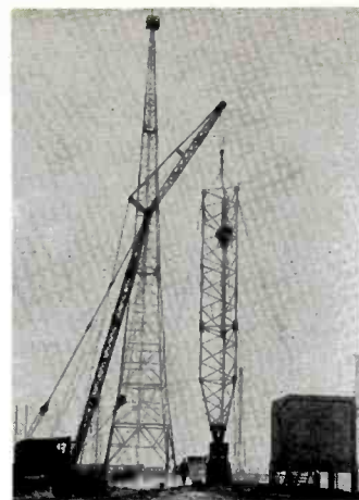
KNBC San Francisco has started work on a new vertical radiator type AM antenna at Belmont, Calif. Transmission is expected to begin before first of year. Transmitter will be 550 feet high on completion and, according to General Manager John Elwood, will add 10,000 square miles to KNBC's primary coverage area.
