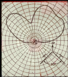
90° angle between dipoles 90° phasing between dipoles
