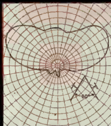
60° angle between dipoles 0° phasing between dipoles
